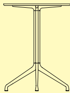
AAT 15 HIGH L80 x W80 x H105 cm
