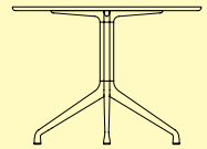
AAT 20 Ø100 x H73 cm
