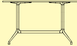
AAT 10 HIGH L160 x W80 x H95 cm
